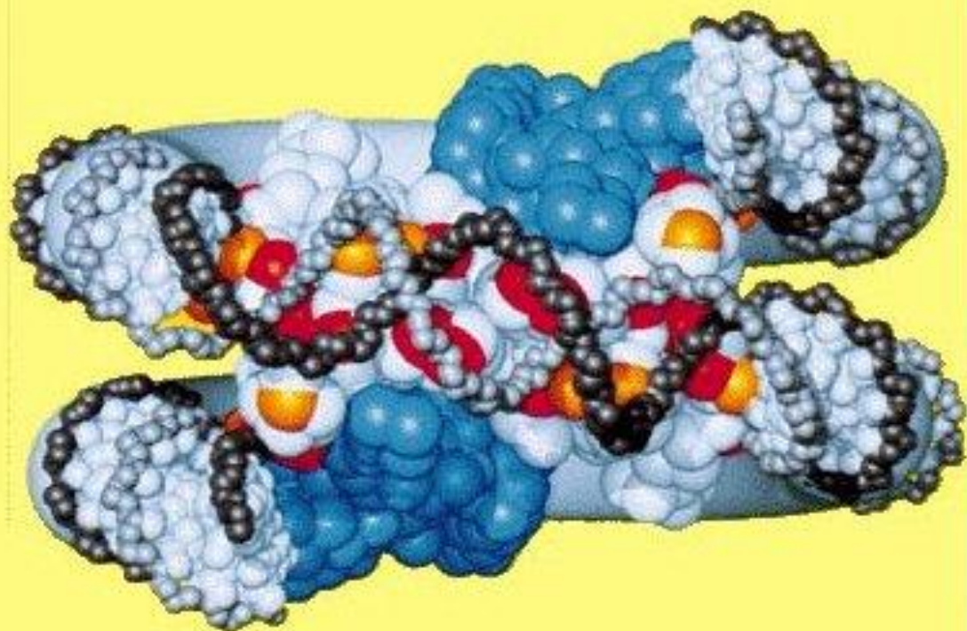
Nucleosome
